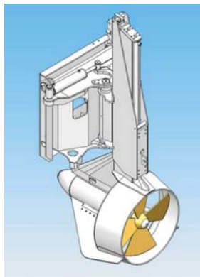
Retractable Unit With Nozzel
