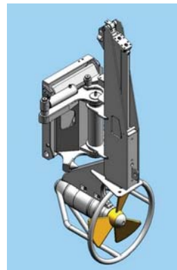
Retractable Unit With Propeller Protection
